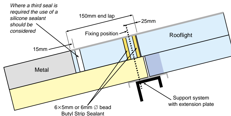
Fig 10: Sandwich panel end lap detail (GRP rooflight over metal)
