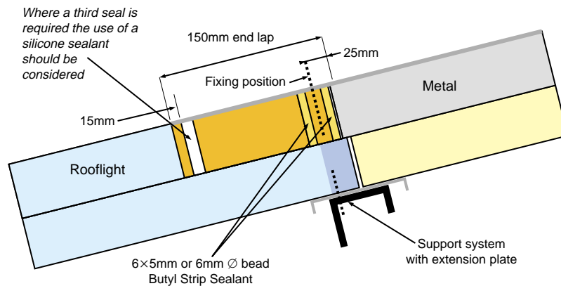
Fig 9: Sandwich panel end lap detail (metal over GRP rooflight)
