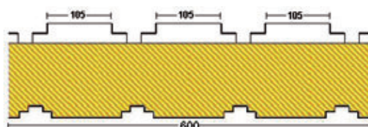
Fig 14: Model constrained by brackets at 600mm centres
