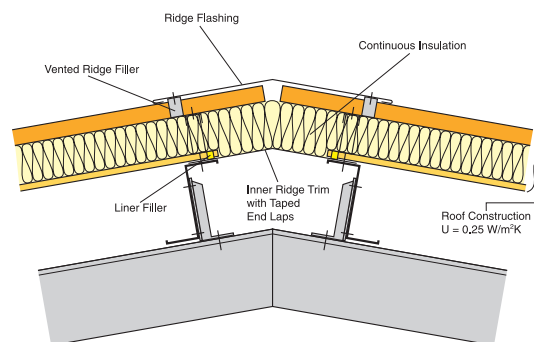
Twin skin
