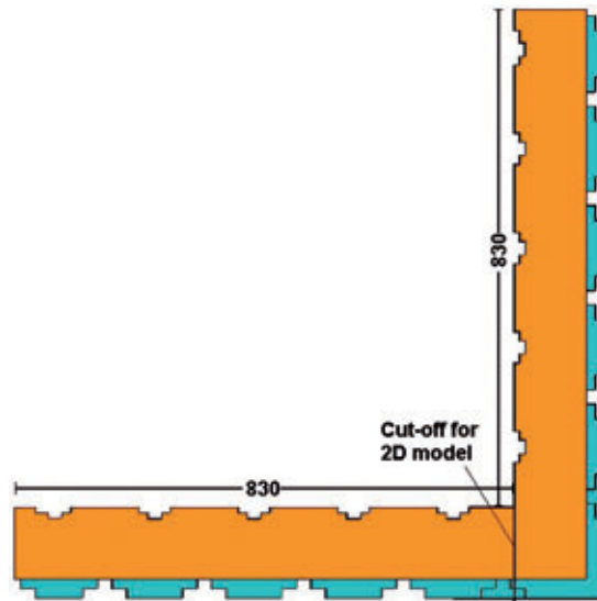
Fig 38: Dimensions of model to calculate the \Psi -value
