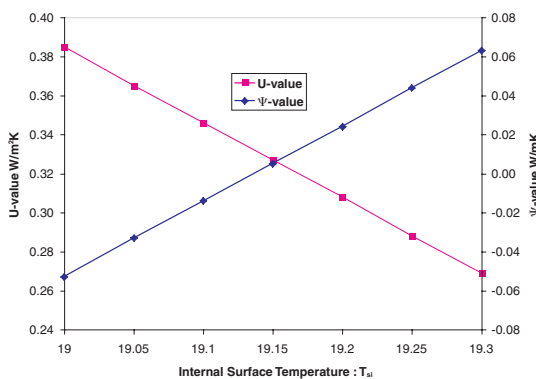
Fig 27: U-value and \Psi -value calculated from T_{si} value
