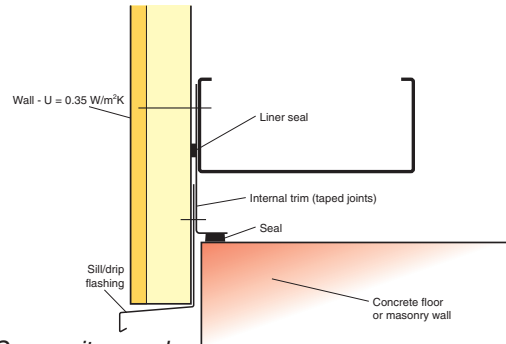
Composite panel
