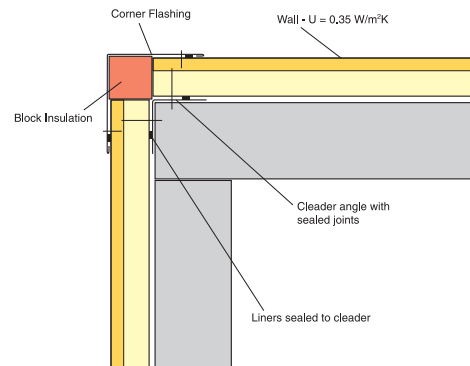
Composite panel
