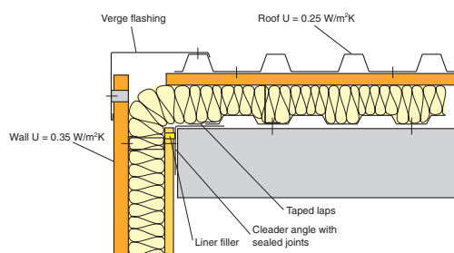
Twin skin
