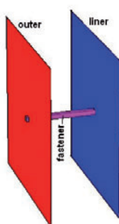
Fastener in composite panel wall (insulation removed)
