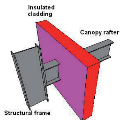
Fig 9: Canopy rafter forming a point thermal bridge
