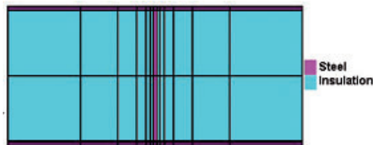
Fig 21 -Two dimensional model of steel crossing insulation – optimum grid
