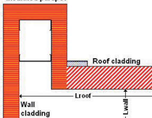
Type 1 parapet verge
